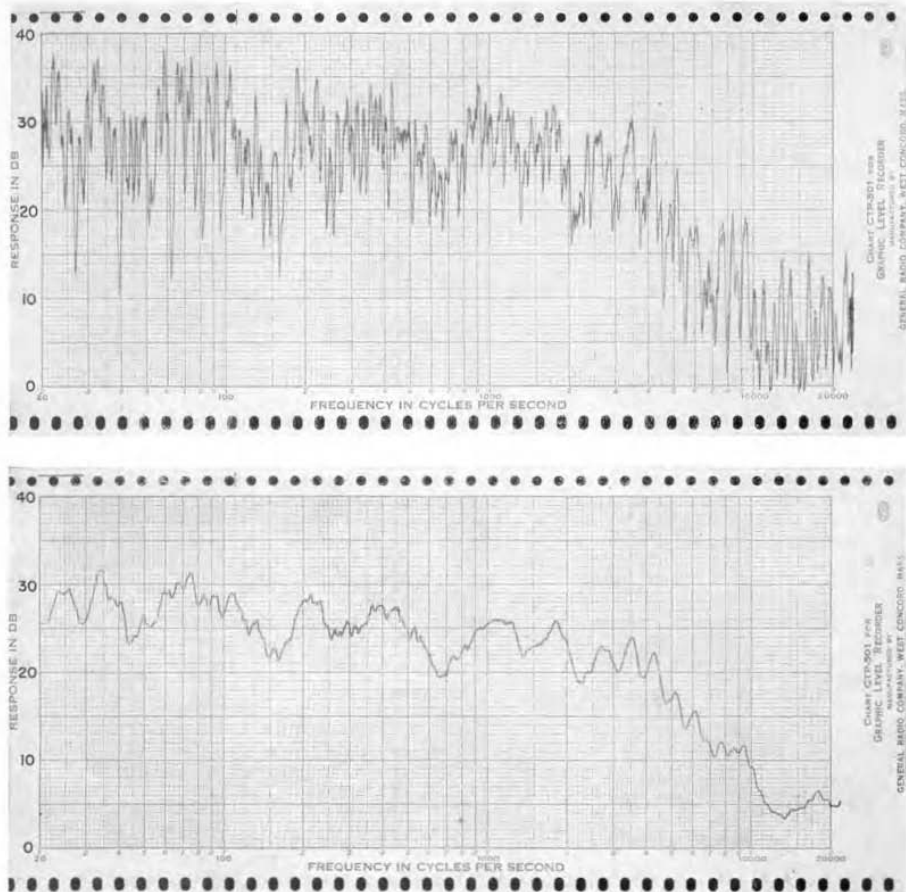
Figure 4. Records of the frequency response of a public address system, taken with (top) maximum writing speed and (below) minimum writing speed.
